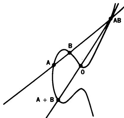
Figure 5.3. Addition of A = (-3, 2) and B = (-1, 4) on the elliptic curve y^2 = x^3 - 7x + 10 , using O = (1, 2) as the zero element. Here AB = (5, 10) and A + B = (-2, -4) .
