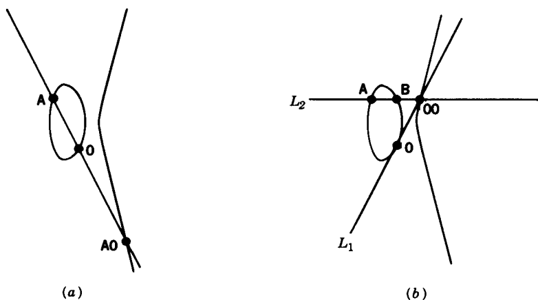
Figure 5.4. The curve y^2 = 4x^3 - 4x + 1 , with A = (-1, 1) , O = (1, 1) . (a) A'O = (2, -5) , O(A'O) = A . (b) OO = (1, 1) , B = A(OO) = (0, 1) , AB = OO , A + B = O(AB) = O(OO) = O .
